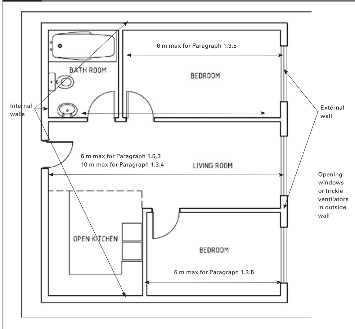
Figure 3: Layout 2 Table 4
