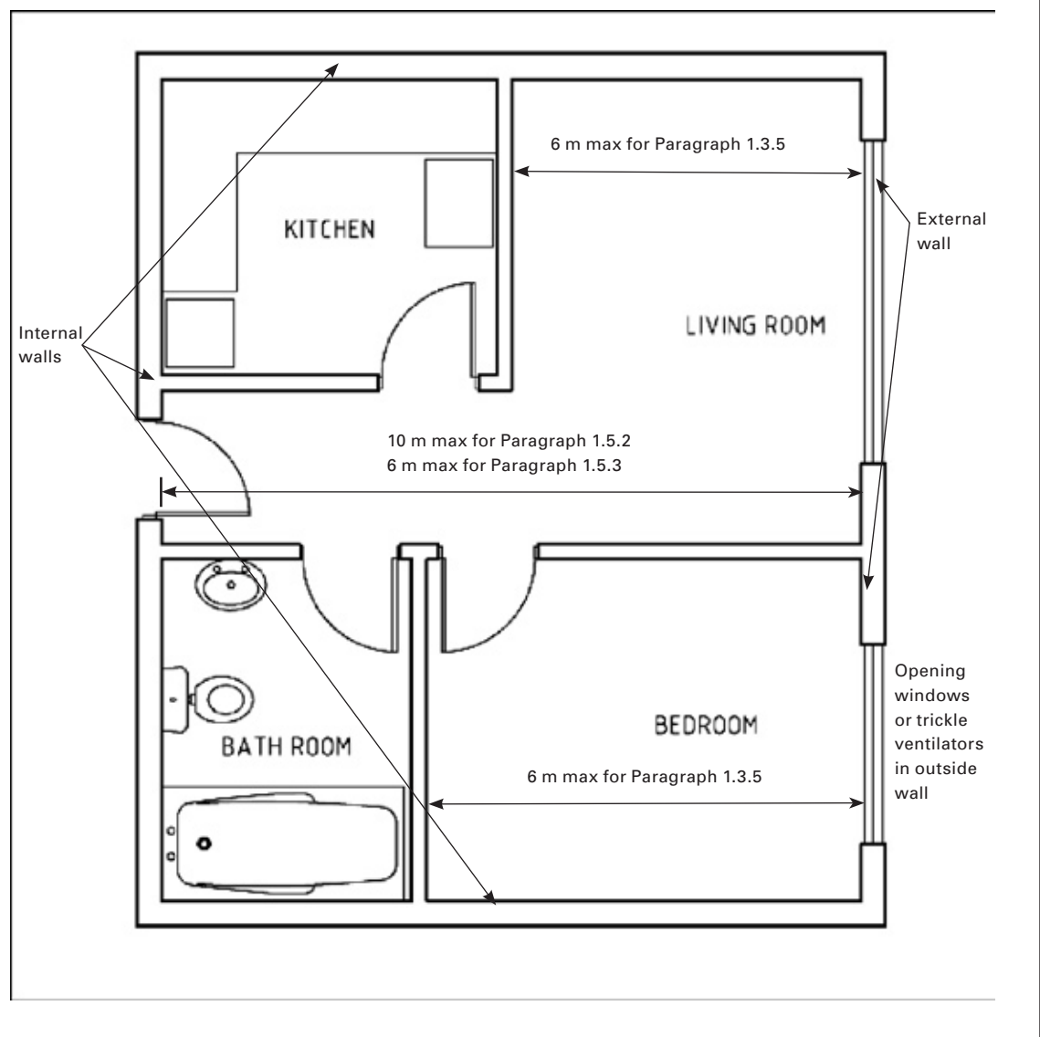
Figure 4: Layout 3 Table 5
